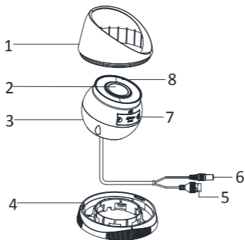
Figure 1-3 Type III Turret Camera Overview
