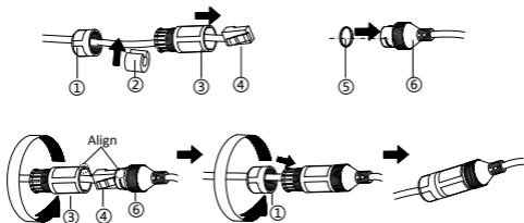
Figure 2-15 Install Waterproof Jacket
