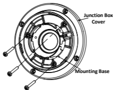
Figure 2-8 Fix Mounting Base
