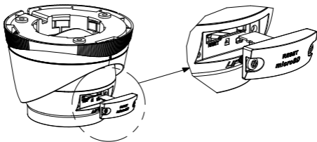
Figure 2-1 Unscrew the Cover and Insert Memory Card
