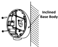
Figure 2-12 Fix the Body of Inclined Base on Ceiling/Wall
