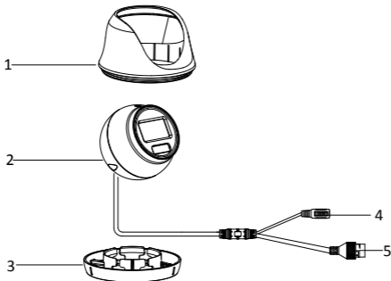
Figure 1-4 Turret Camera Overview
