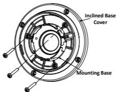
Figure 2-11 Fix Mounting Base
