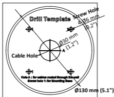
Figure 2-7 Drill Template
