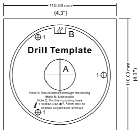
Figure 2-2 The Drill Template
