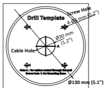
Figure 2-10 Drill Template
