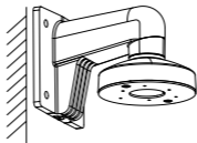
Figure 2-13 Install the Wall Mounting Bracket
